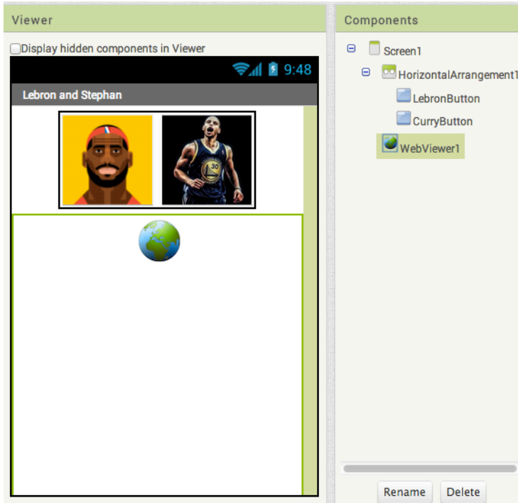
Figure 24-3. The WebView as it appears in Designer.
